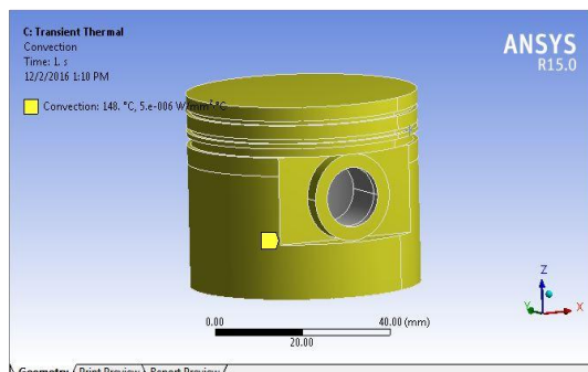
Convection applied on piston side wall
