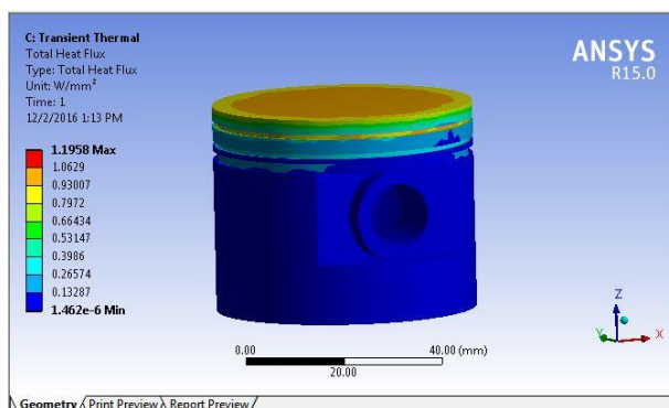
Max. Heat flux for Graphite piston
