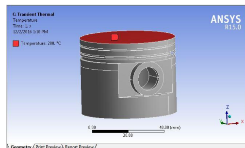
Temperature applied on piston head
