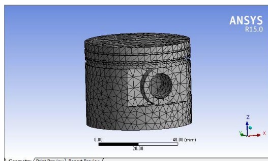
Meshing of piston with Triangular element
