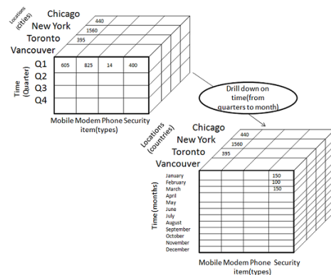
Fig. 3. Drill Down Operation
