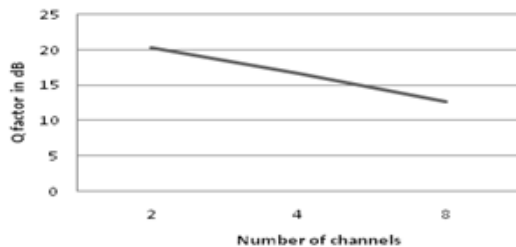
Fig. 10:Q factor Vs number of channels
