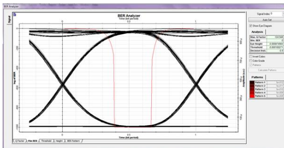
Fig. 5b: Min. BER for 95 GHz channel spacing
