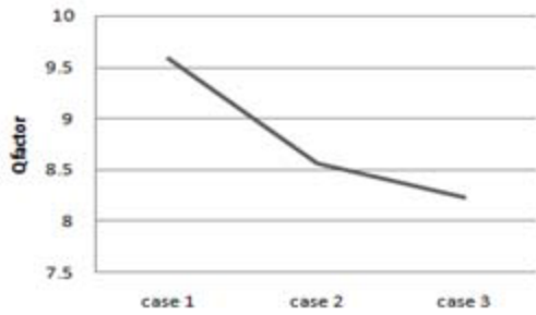
Fig. 8: Q- factor measured with unequal channel spacing
