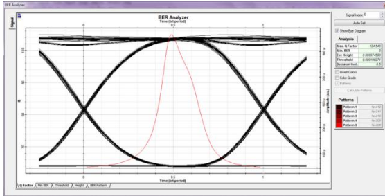
Fig. 5a: Q-factor for 95 GHz channel spacing
