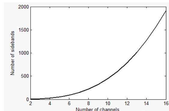
Fig. 2: Number of FWM sideband
