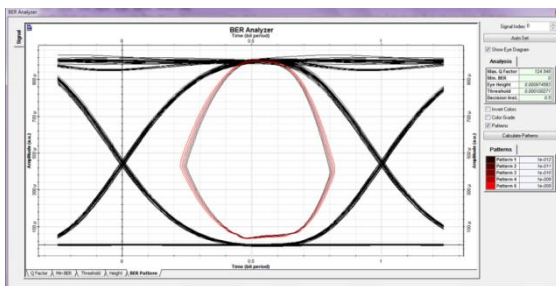
Fig. 5c: Eye Pattern for 95 GHz channel spacing
