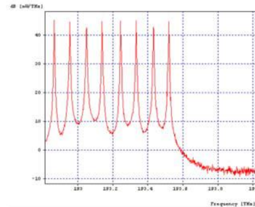
Fig. 4a: Input Pattern for 95 GHz channel spacing
