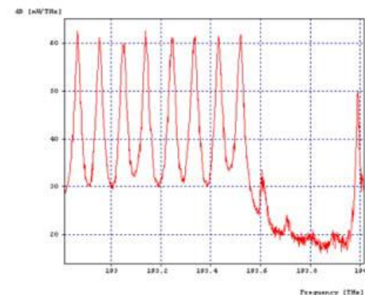
Fig. 4b: Output Pattern for 95 GHz channel spacing
