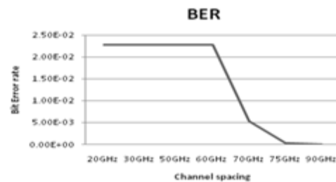
Fig.6 : BER factor Vs channel spacing
