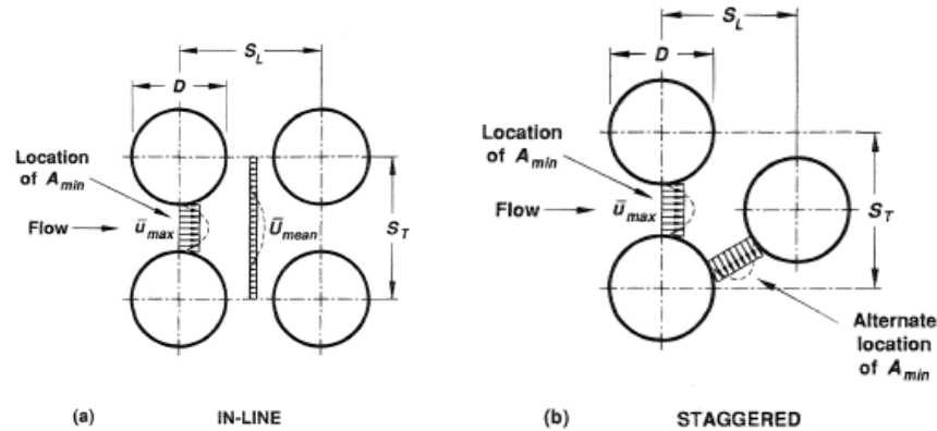
Figure 1 Schematic of (a) an in-line and (b) a staggered tube bank illustrating nomenclature, and showing location of minimum cross section
