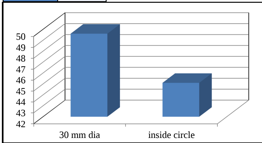
Figure-13 Graphical comparison of the temperatures obtained for the two cases
