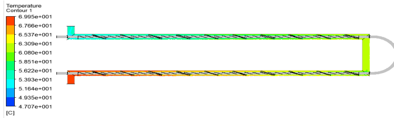
Figure 13: Hot fluid temperature contour
