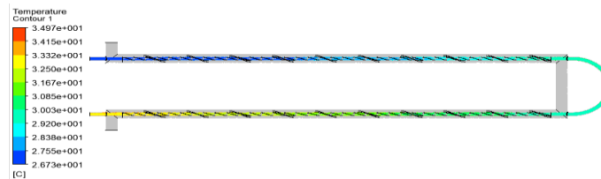
Figure 14: cold fluid temperature contour
