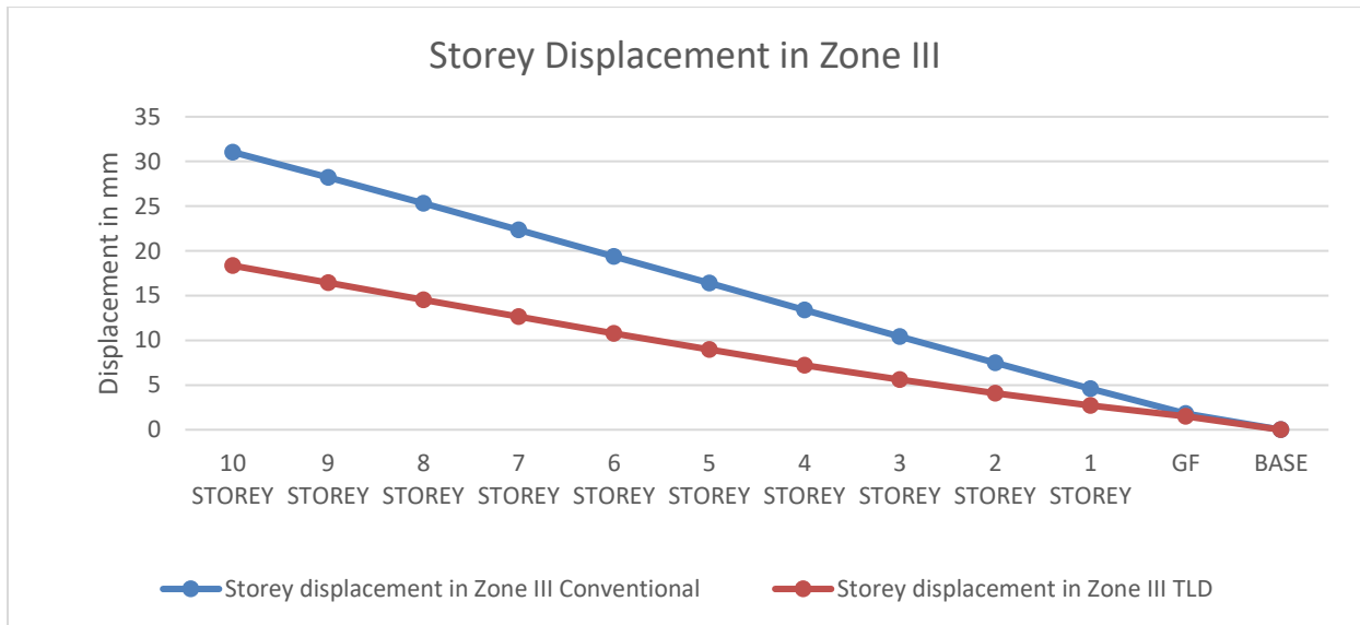
Figure 6 Storey Displacement in Zone III
