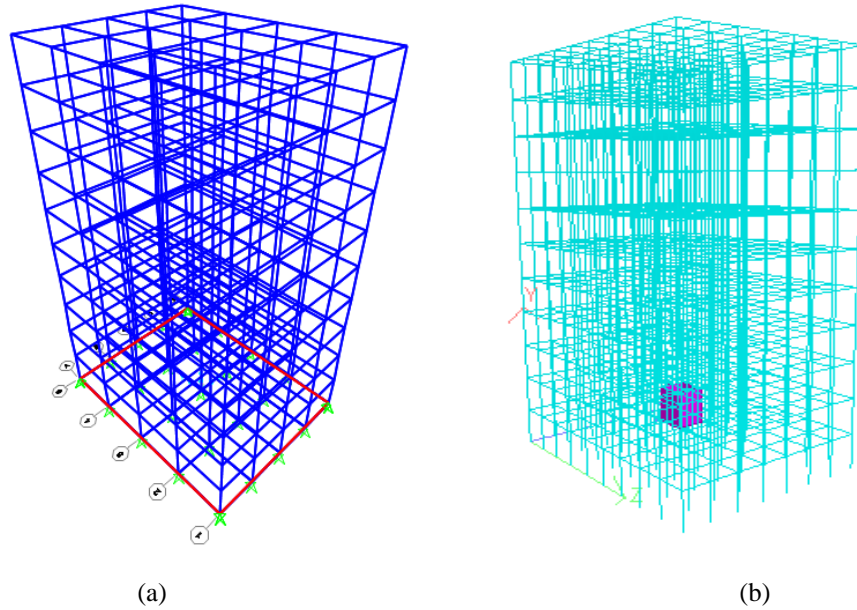
Figure 1 (a) Model of the Building (b) Building with Tuned Damper
