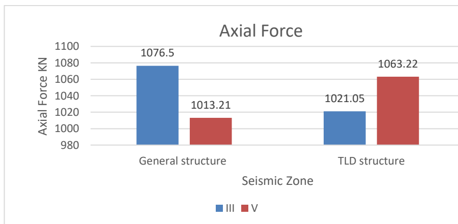
Figure 5 Max. Axial Force (KN)
