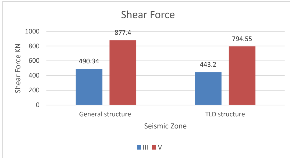
Figure 4 Max. Shear Force
